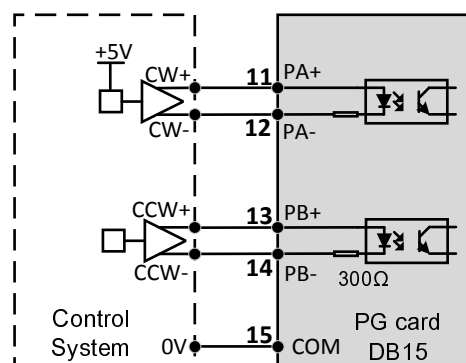
Figure 4 Differential pulse is given wiring diagram
