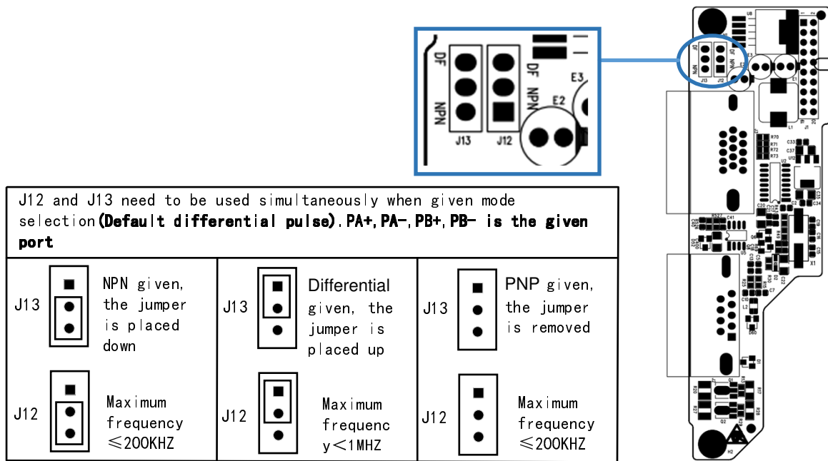
Figure 2 Control System Pulse Given Selection
