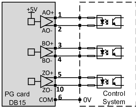
Figure 6 Differential pulse divider output wiring diagram
