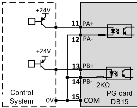
Figure 5 PNP pulse given wiring diagram
