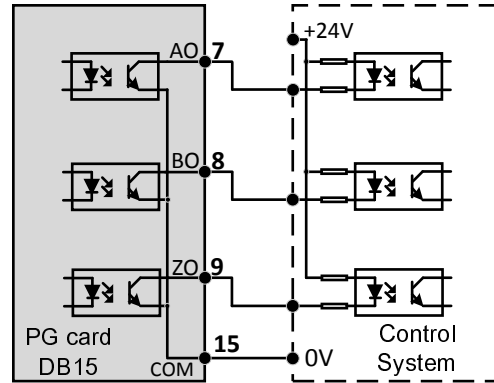
Figure 7 NPN pulse divider output wiring diagram
