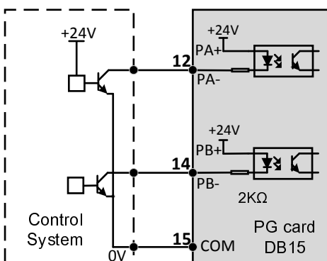
Figure 3 NPN pulse given wiring diagram
